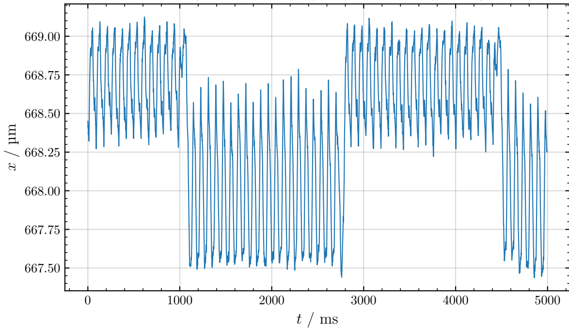
micromer-M (12.50 Hz, 20 ms): particle ID 5 (rank 6/14275)
